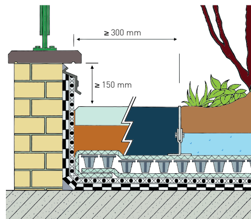
Detail 1. Parapet
