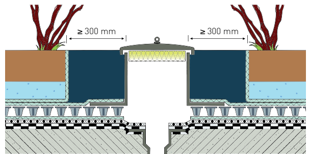
Detail 5. Roof outlet
