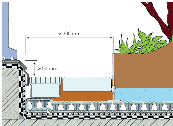
Detail 4. Door threshold
