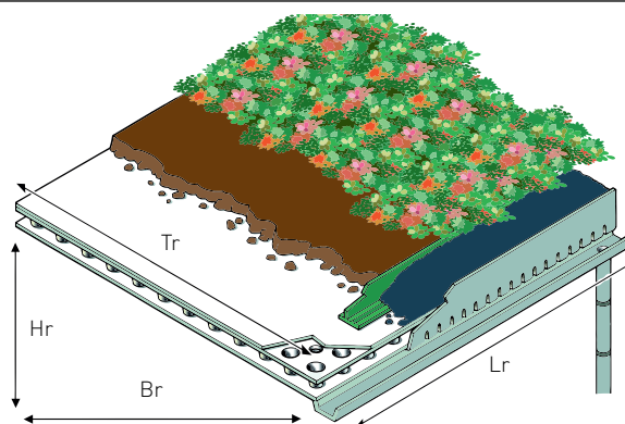
Figure 1. Roof dimensions
