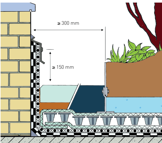
Detail 3. Facade with an opening
