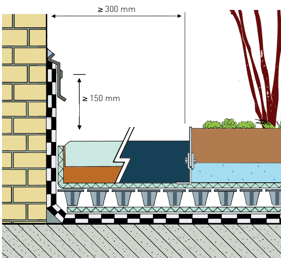
Detail 2. Facade
